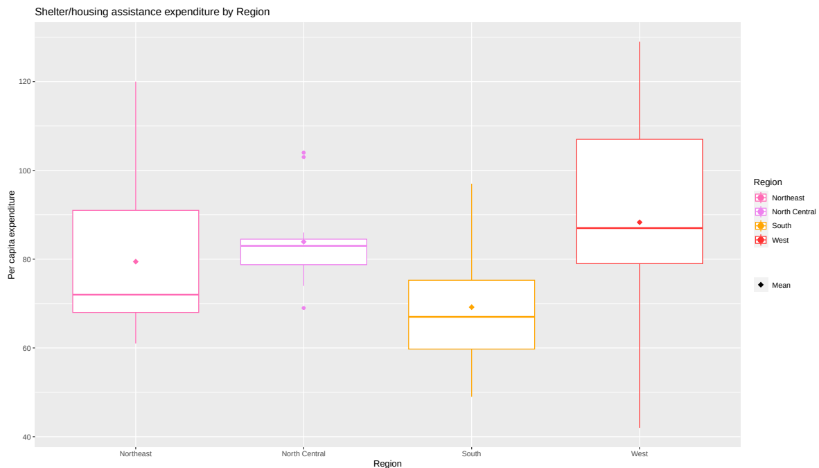
Figure 3: Boxplot of expenditure on shelter/housing assistance colour-coded by Region
