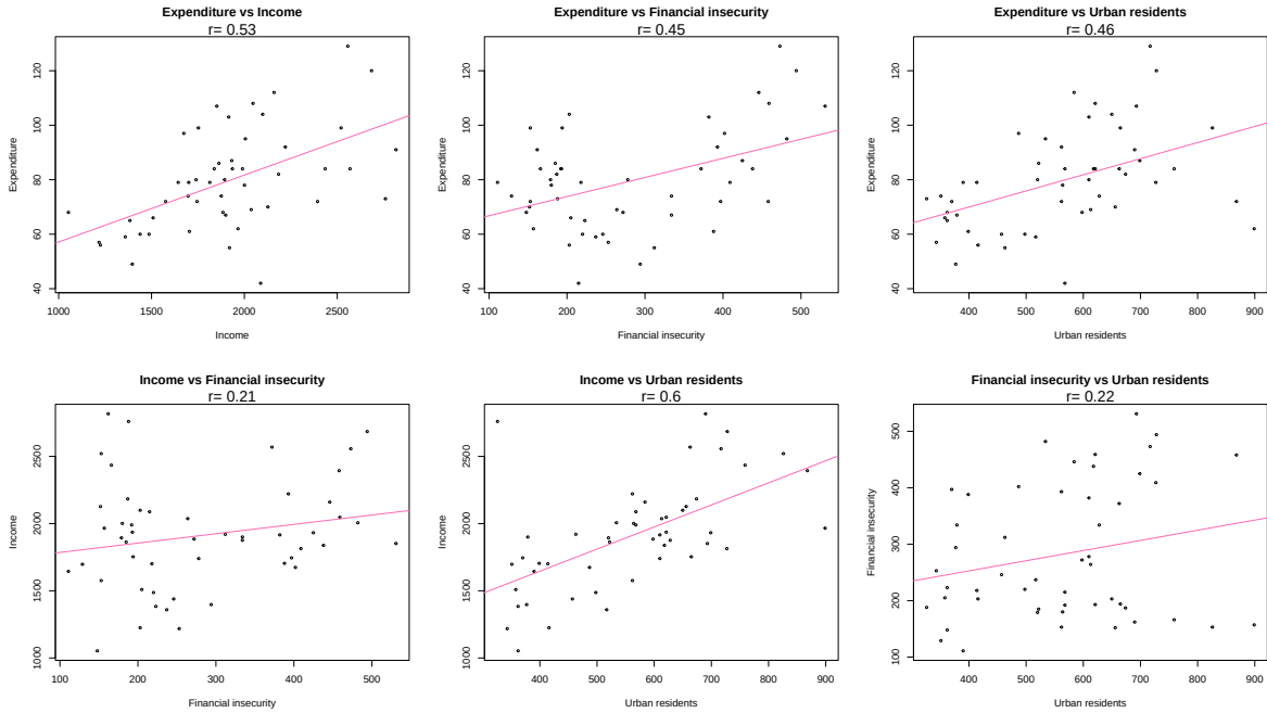
Figure 2: Six scatterplots showing the relationships among expenditure, income, financial insecurity, and urban residents
