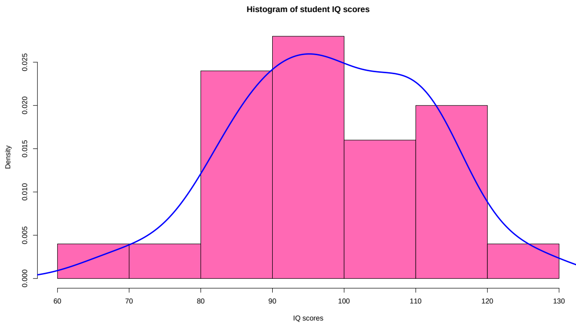
Figure 1: Histogram showing the normal distribution of dataset "y"
